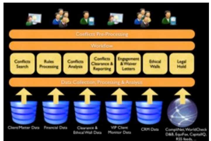
Compliguard Analyze Service Oriented Architecture
