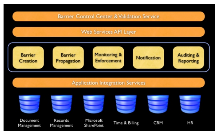
Compliguard Protect Service Oriented Architecture
