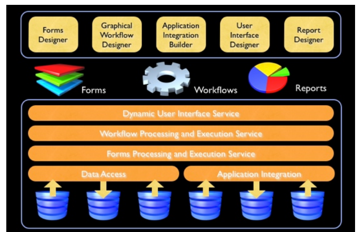
Compliguard Flow Service Oriented Architecture
